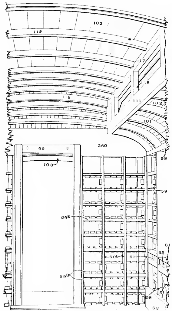
Fig. 538. Interior View.
